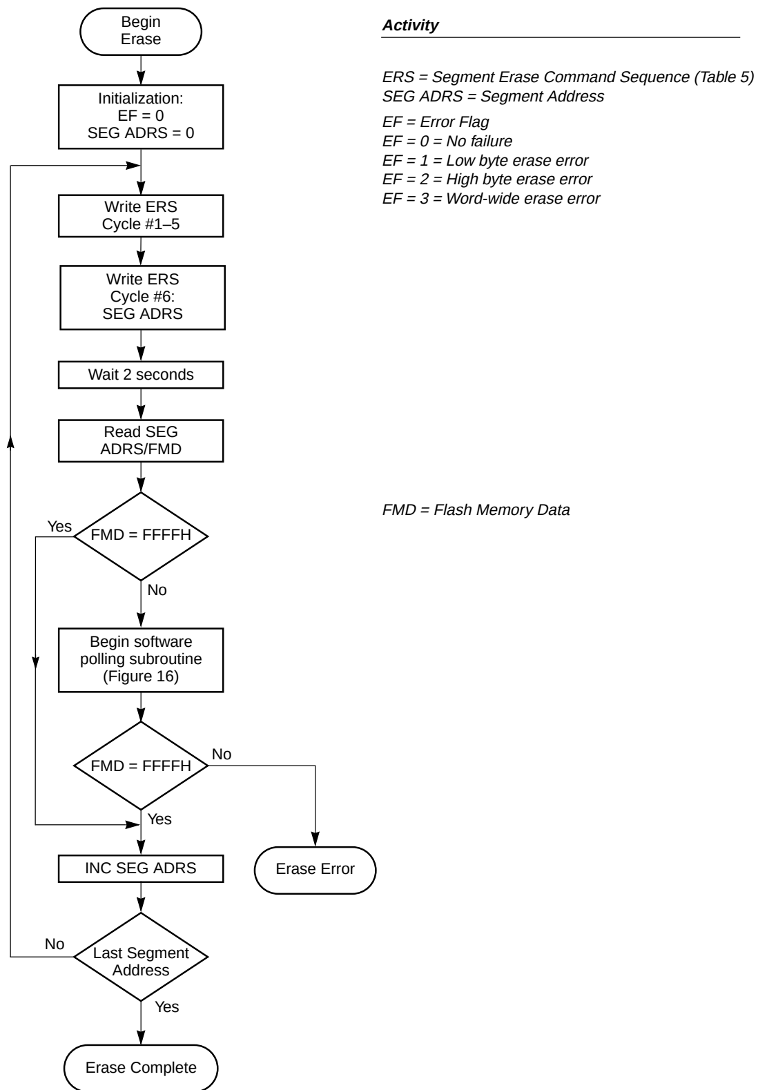
Figure 15. Word-Wide Erasure Flow Chart
