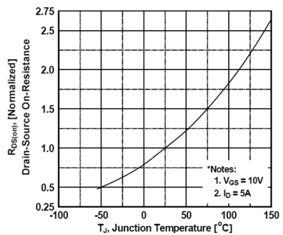
Fig.2 On-Resistance Variation vs Temperature
