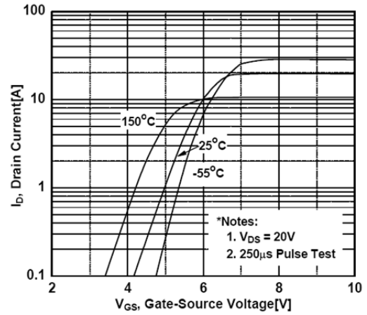
Fig. 4 Transfer Characteristics
