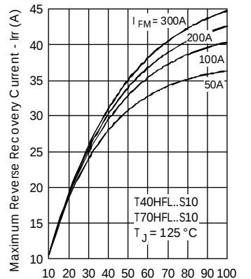
Fig. 27 - Recovery Current Characteristics
