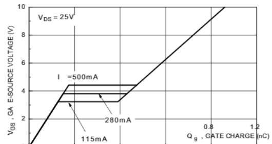
Figure 10. Gate Charge Characteristics
