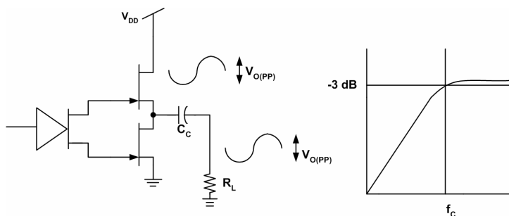
Figure 40. Single-Ended Configuration and Frequency Response
