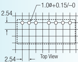
Recommended Footprint Details
