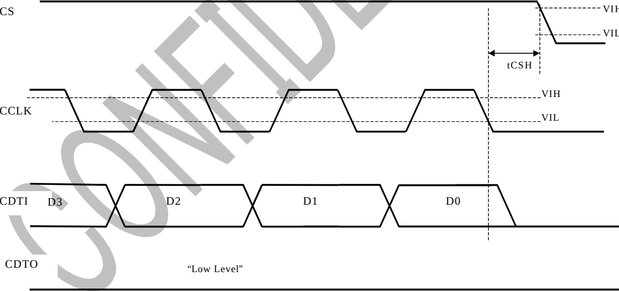
Figure 4. Control Data Interface Timing (Write Timing)
