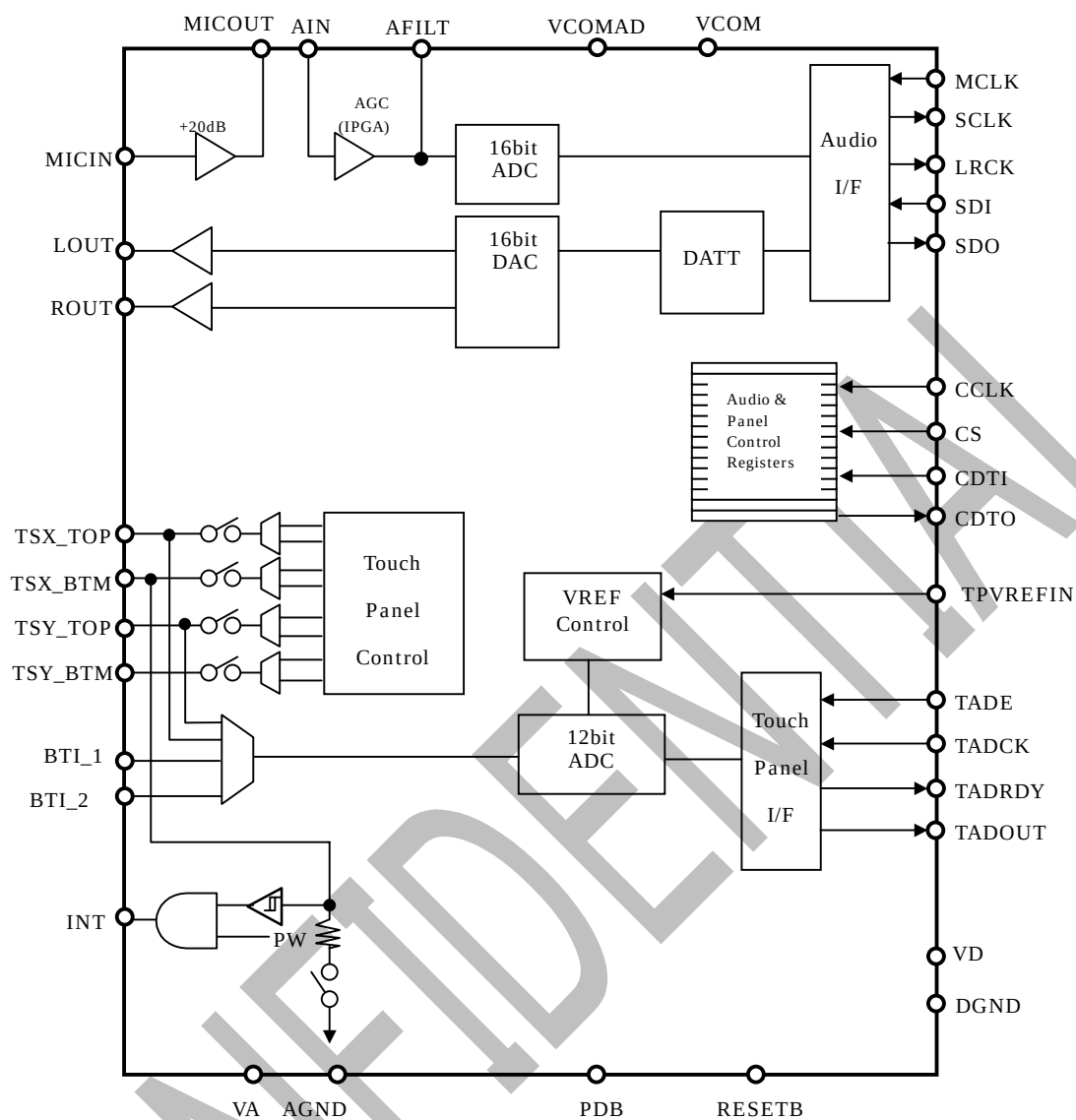
BLOCK DIAGRAM
