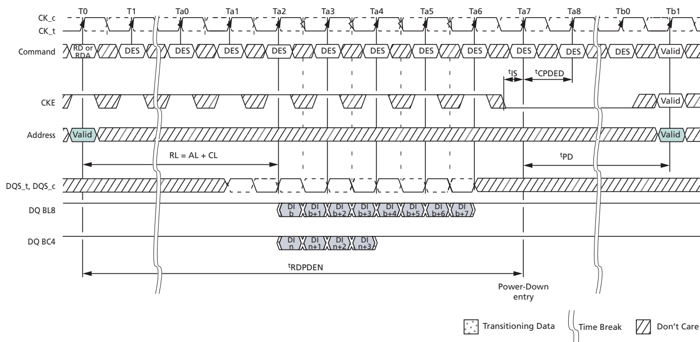
Figure 93: Power-Down Entry After Read and Read with Auto Precharge
