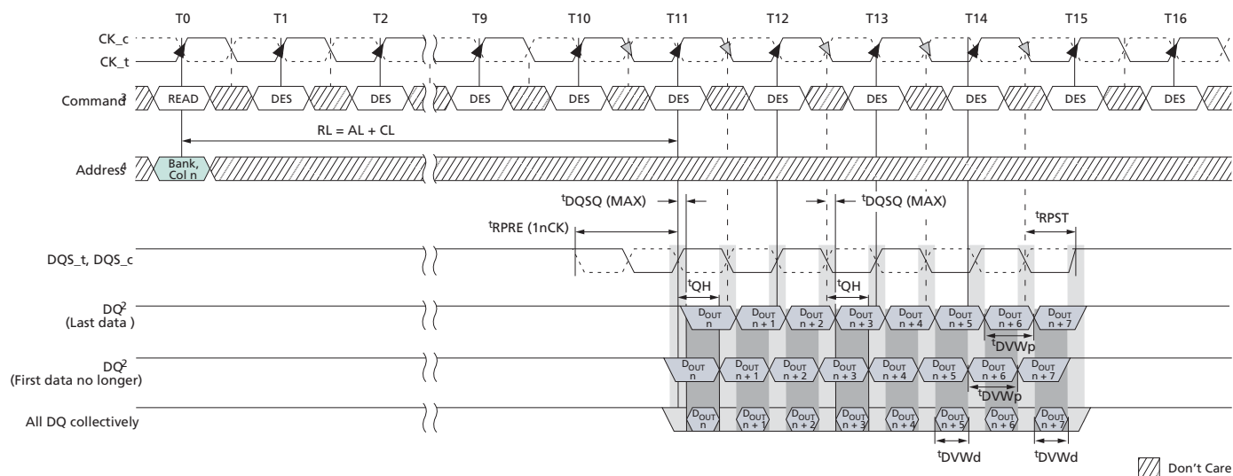
Figure 125: Data Strobe-to-Data Relationship
