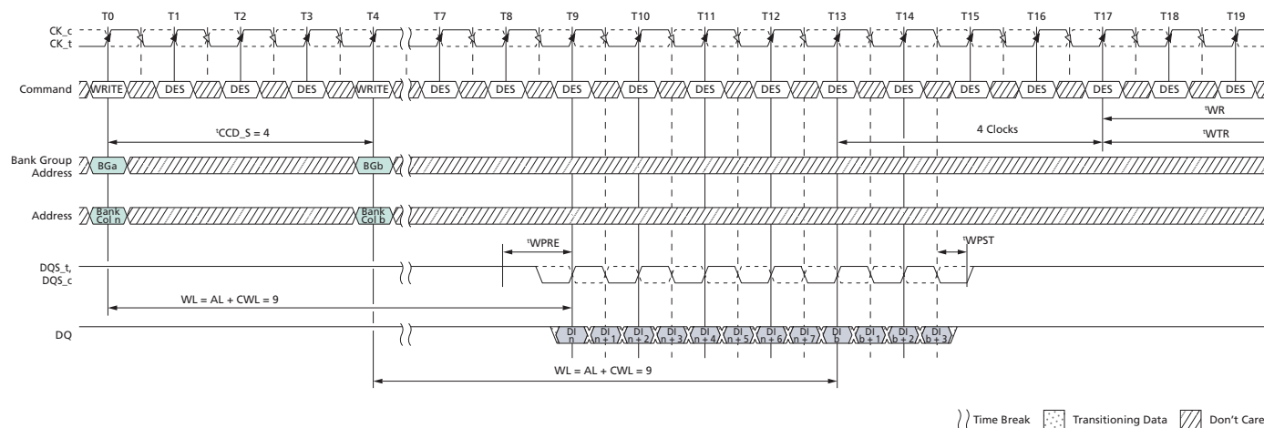
Figure 180: WRITE (BL8) to WRITE (BC4) OTF with 1^{\text{st}} CK Preamble in Different Bank Group
