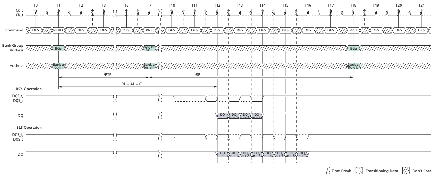
Figure 152: READ to PRECHARGE with 2 t CK Preamble
