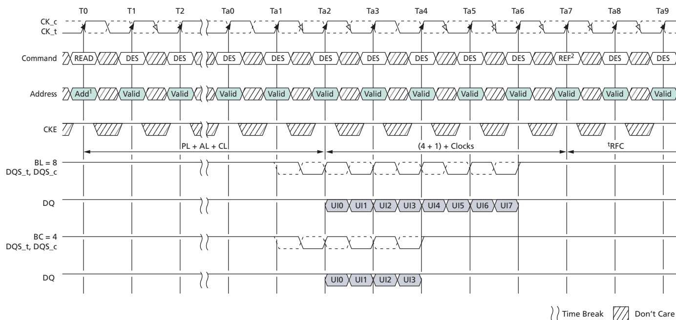
Figure 41: READ-to-REFRESH Timing
