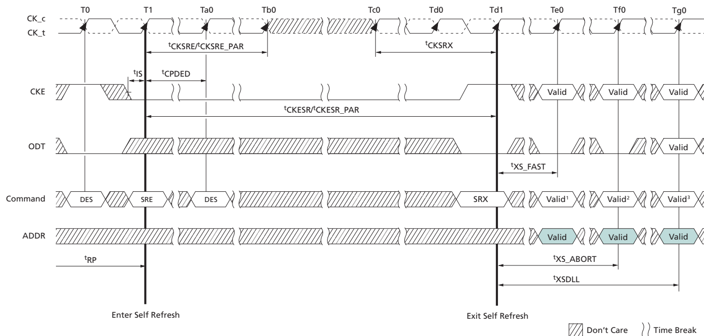
Figure 90: Self Refresh Abort
