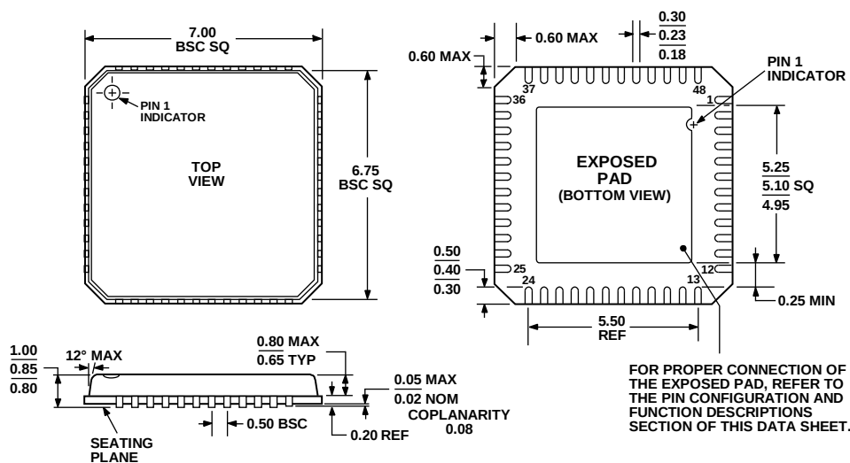
Figure 40. 48-Lead Lead Frame Chip Scale Package [LFCSP_VQ] 7 mm x 7 mm Body, Very Thin Quad (CP-48-1) Dimensions shown in millimeters
