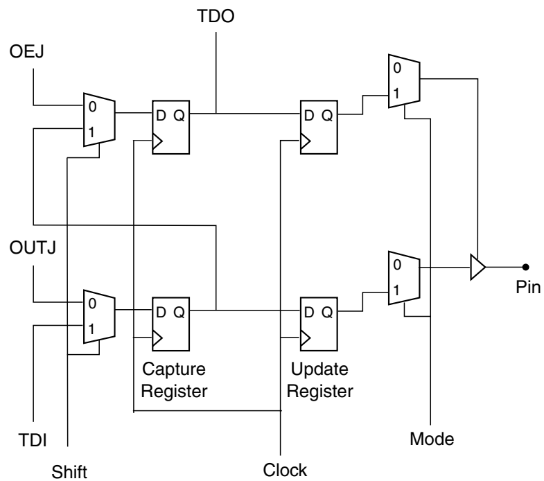
Macrocell BSC
