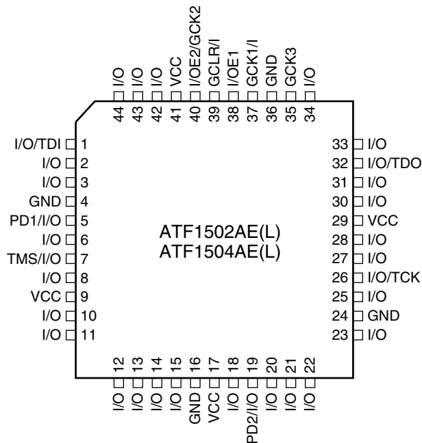
44-lead TQFP
