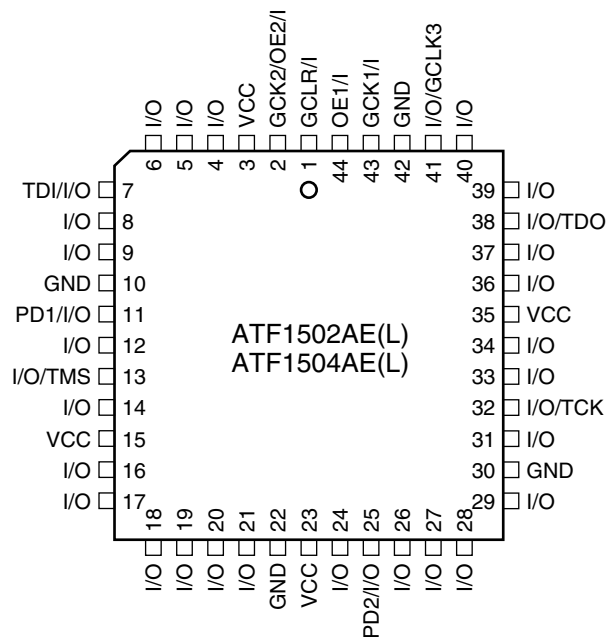
44-lead TQFP
