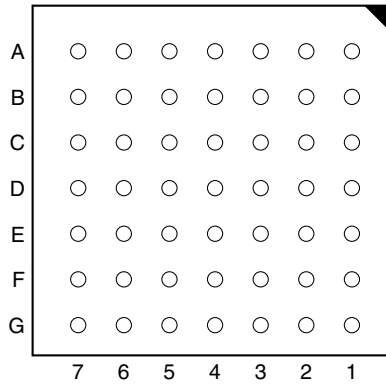
ATF1504AE(L) 49-ball 0.8 mm Pitch Bottom View
