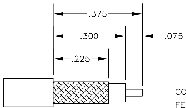
STRIPPING DIMENSIONS
