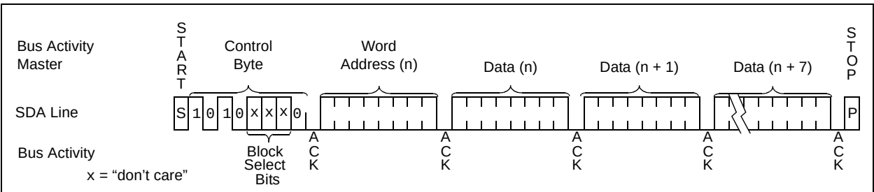
FIGURE 5-2: PAGE WRITE
