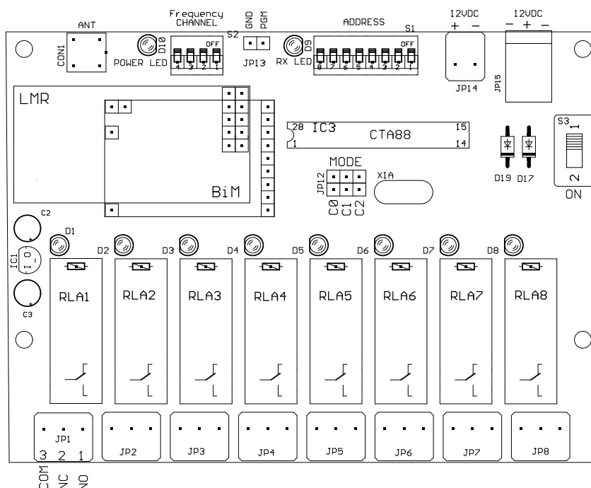
Figure 4: CTA88 Decoder application board for BiM / LMR Receiver
