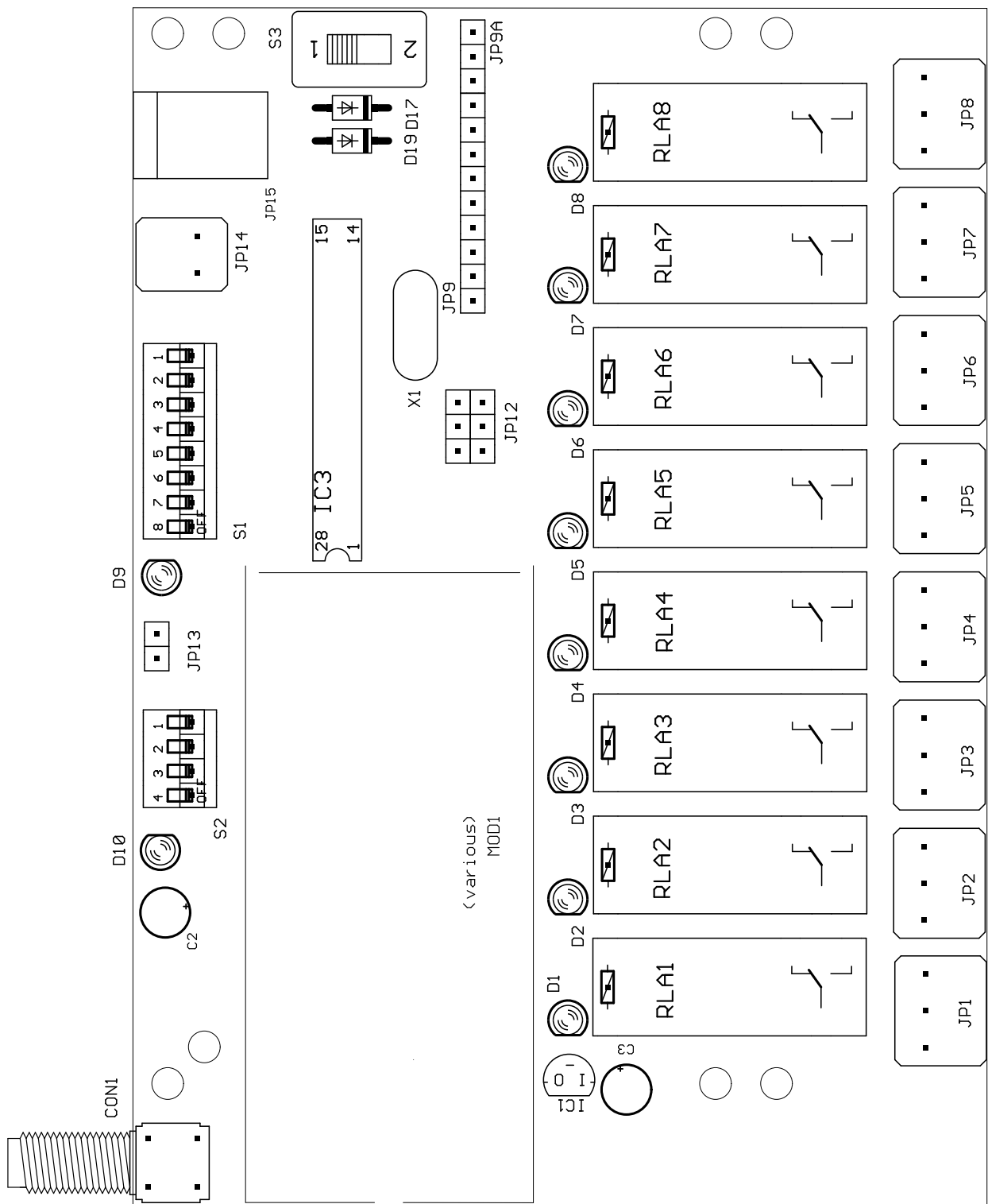
Figure 12: CTA88 Decoder application board for SHX1R / UHX1R / FPX3R Receiver
