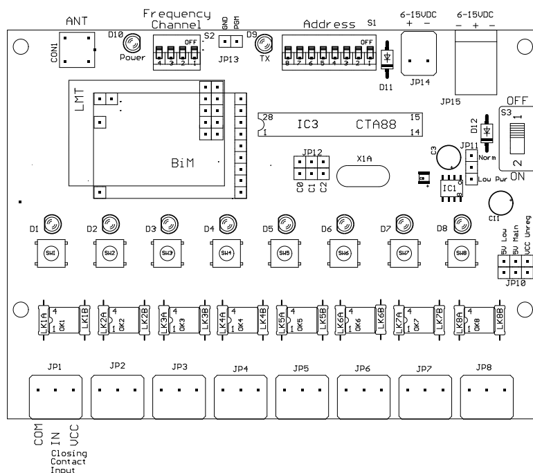
Figure 3: CTA88 Encoder application board for BiM / LM Transmitter
