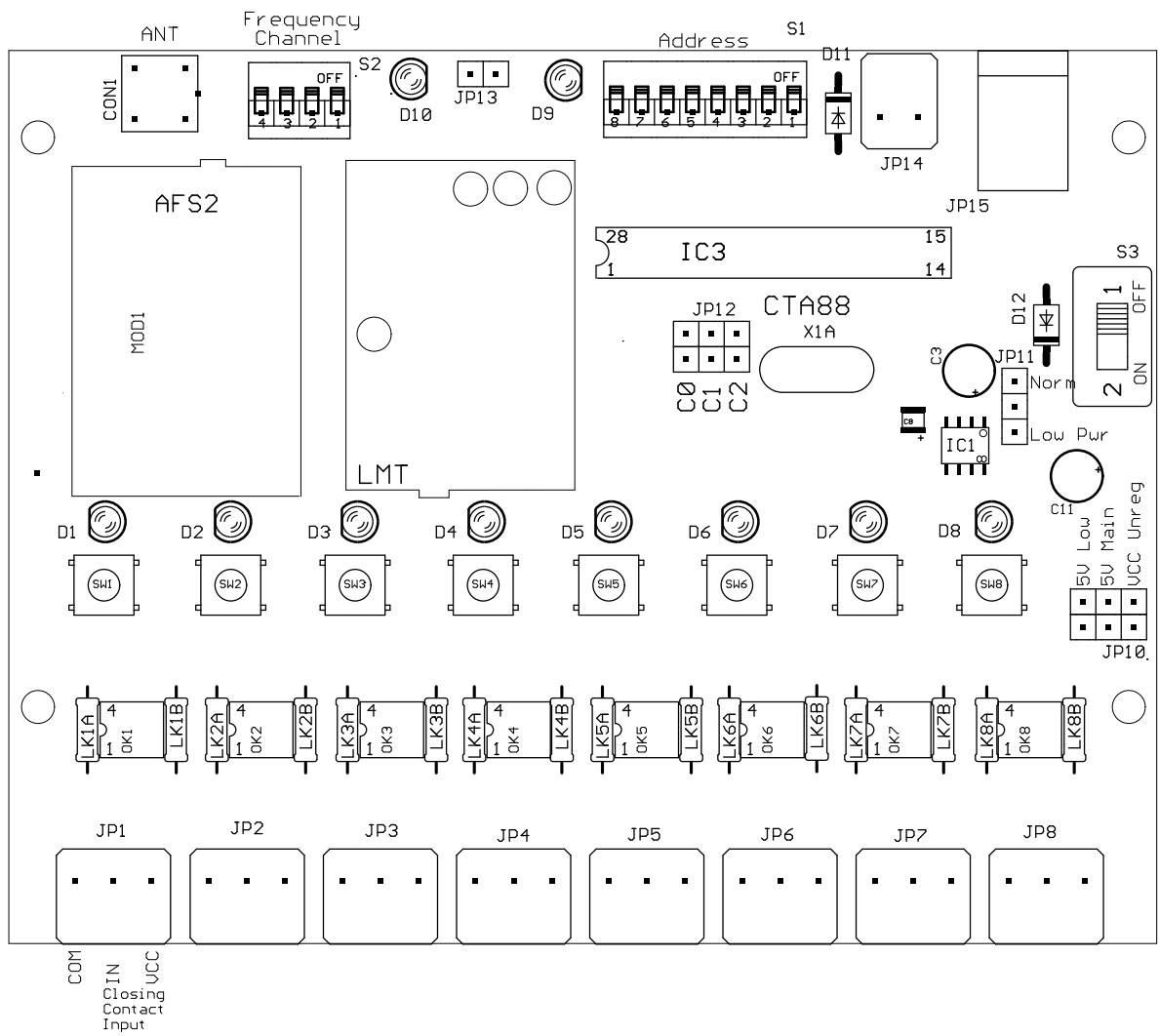
Figure 8: CTA88H Encoder application board for AFS2 Amplifier, LMT2 Transmitter
