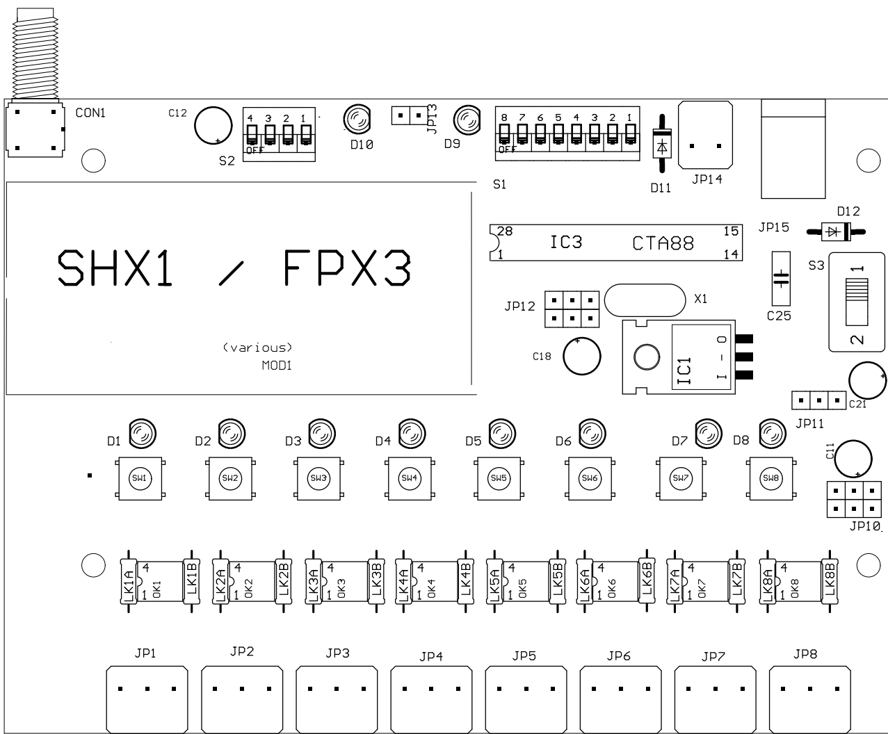
Figure 10: CTA88 Encoder application board SHX1T / UHX1T / FPX3T Transmitter
