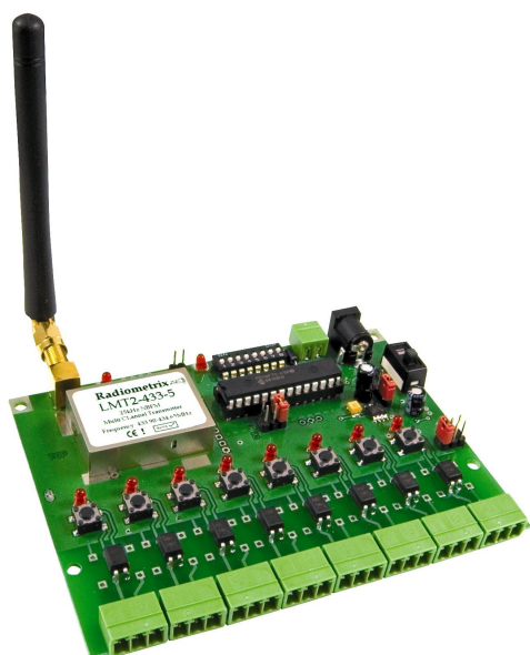
Figure 2: CTA88 TX application board
