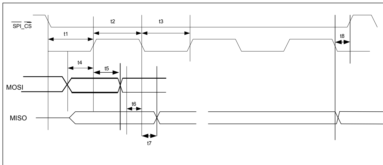
Figure 11-13 EEPROM Interface Timing
