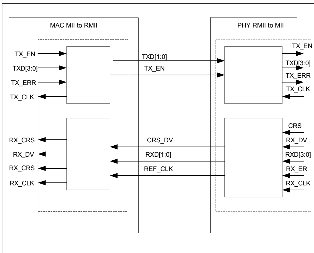
Figure 8-7 RMII Interface
