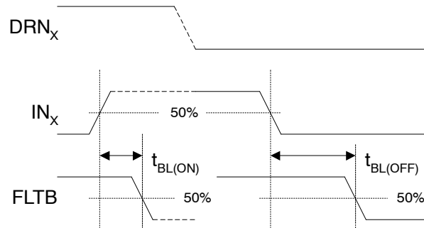
Figure 6. Blanking Timing Diagram
