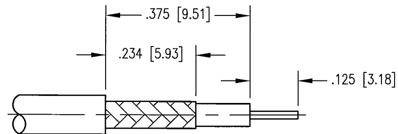
CABLE TRIMMING DIMENSIONS
