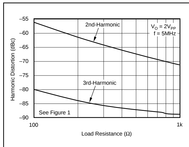
FIGURE 15. 5MHz Harmonic Distortion vs Load Resistance.
