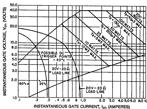
GATE CHARACTERISTICS
