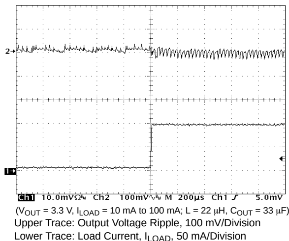
Figure 25. Load Transient Response for V_{IN} = 2.4 \text{ V}
