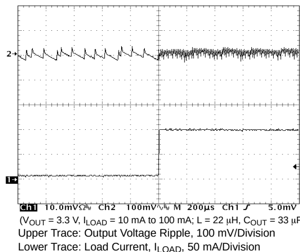
Figure 26. Load Transient Response for V_{IN} = 3.3 \text{ V}
