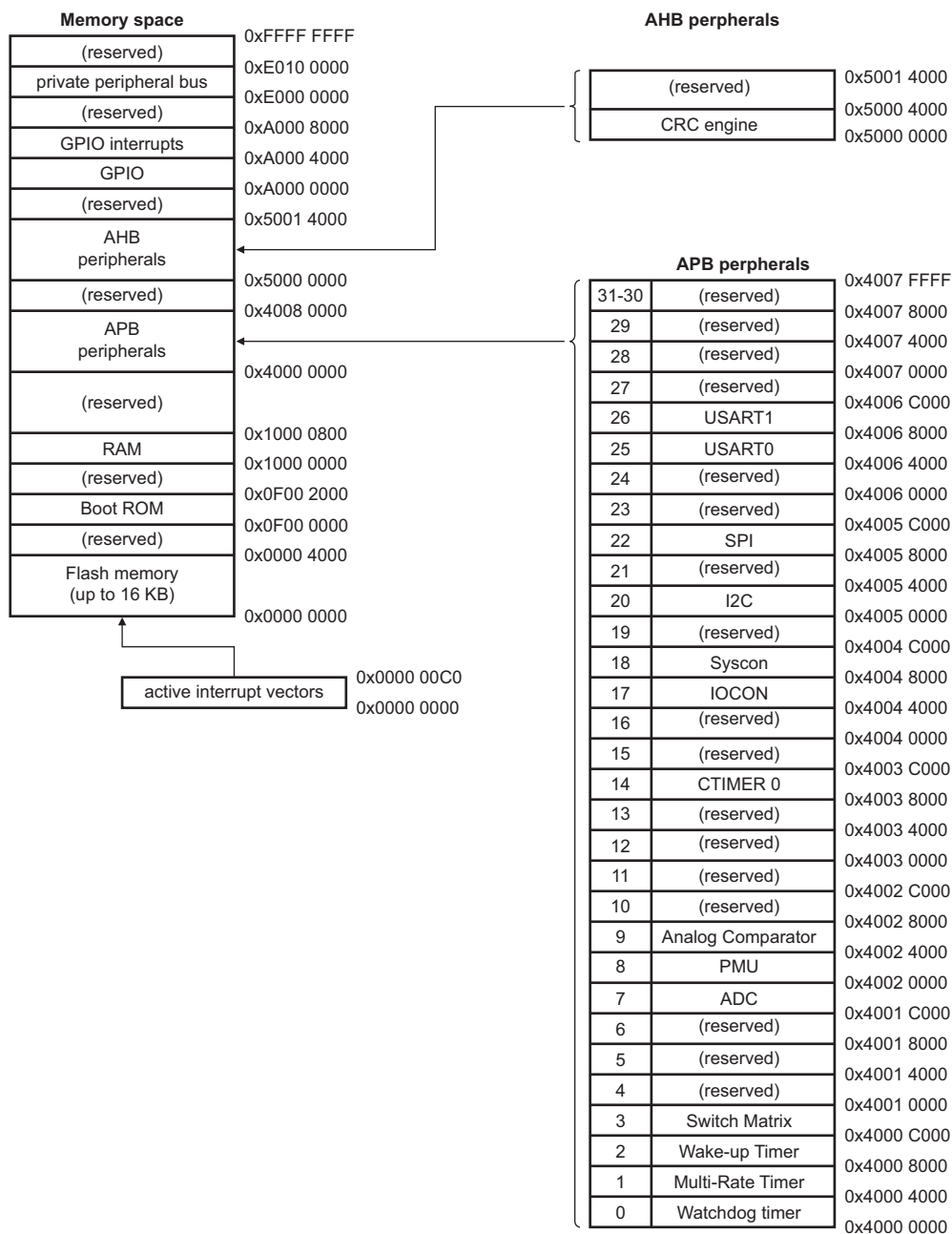
Fig 9. LPC802 Memory mapping
