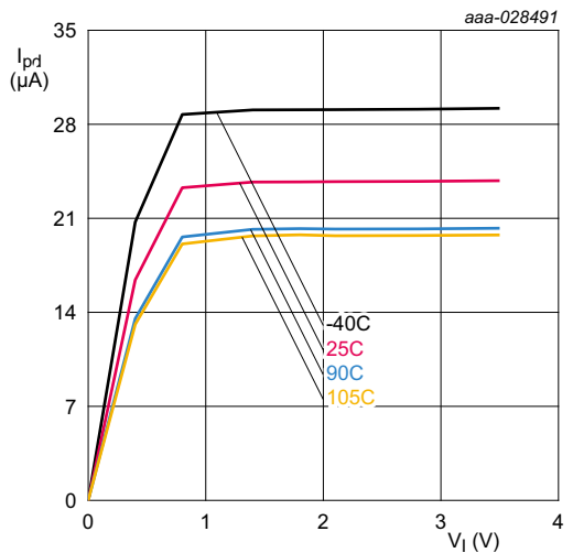
Fig 25. Typical pull-down current I_{PD} versus input voltage V_I
