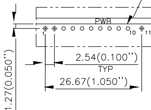
RECOMMENDED PWB LAYOUT
