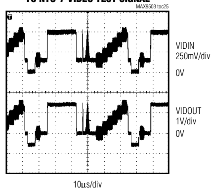
MAX9503M OUT RESPONSE TO NTC-7 VIDEO TEST SIGNAL
