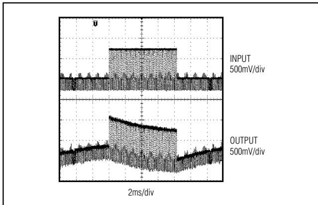
Figure 1. AC-Coupled Output
