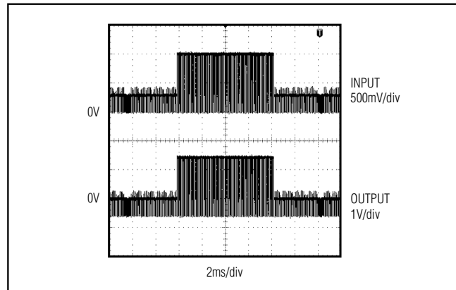
Figure 2. DirectDrive Output
