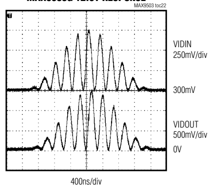
MAX9503G 12.5T RESPONSE
