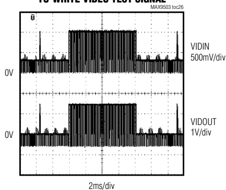
MAX9503G OUT RESPONSE TO BLACK-TO-WHITE VIDEO TEST SIGNAL
