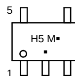
SC-88A
