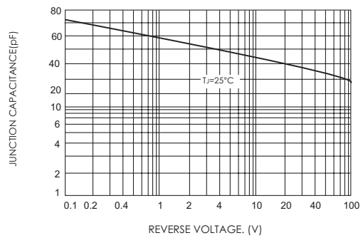
FIG.4-TYPICAL JUNCTION CAPACITANCE
