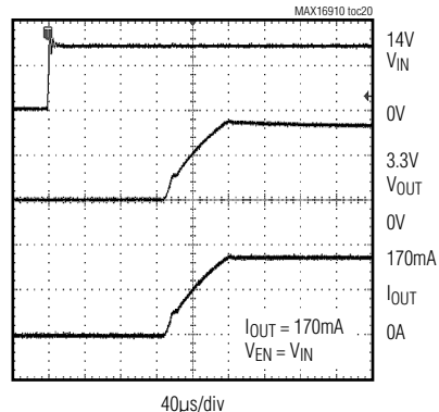
POWER-UP RESPONSE
