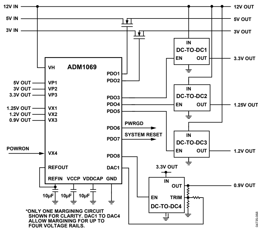
Figure 34. Applications Diagram
