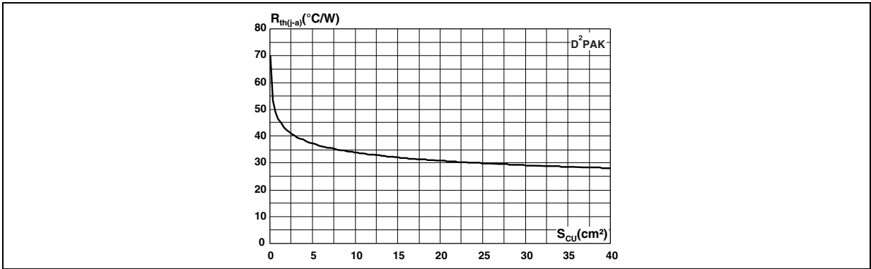
Figure 11. Thermal resistance junction to ambient vs. copper surface under tab (D 2 PAK, printed circuit board FR4, copper thickness: 35 µm)
