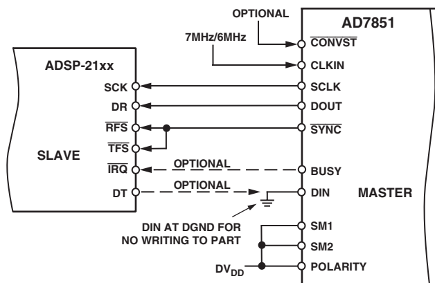
Figure 47. ADSP-21xx Interface
