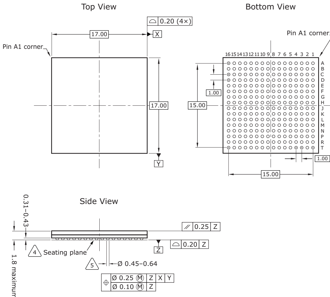
Figure 83 • Package Drawing
