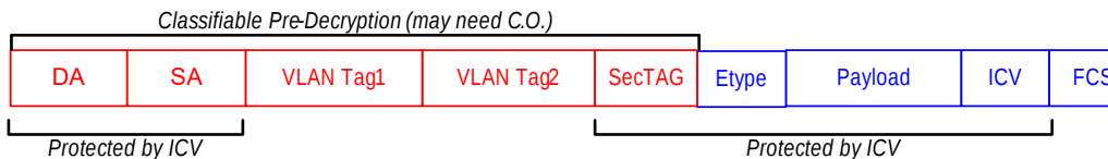
Figure 32 • EoMPLS with One Label
