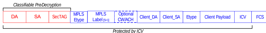
Figure 33 • Standard and Advanced MACsec Transform
