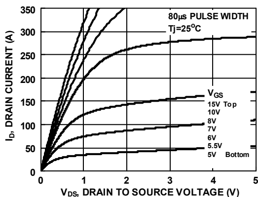
Figure 9. Saturation Characteristics
