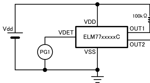
5) Delay time 1 & release time 1
