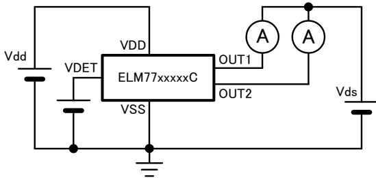
3) Output current & leakage current
