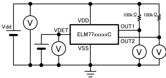
1) Detection voltage & hysteresis width
