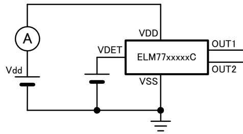
2) Current consumption
