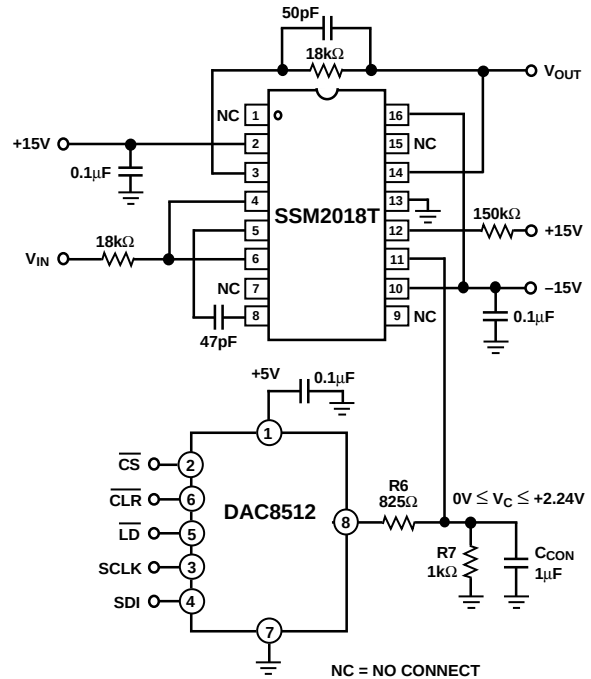
Figure 44. 12-Bit DAC Controls the VCA Gain
