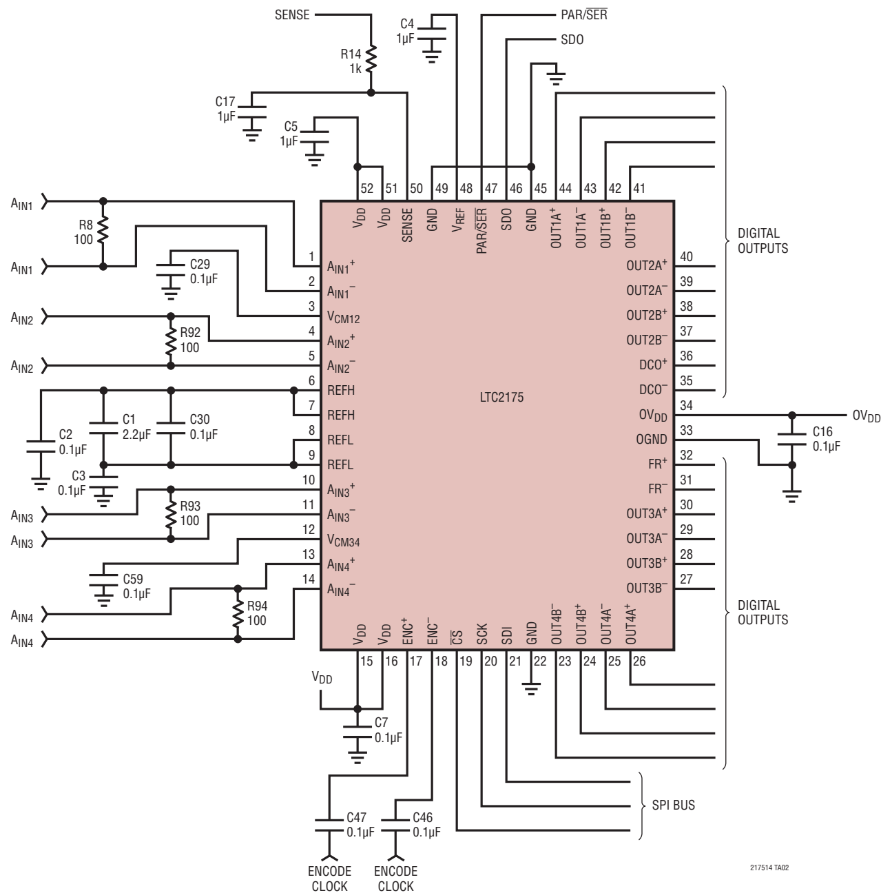
LTC2175 Schematic
