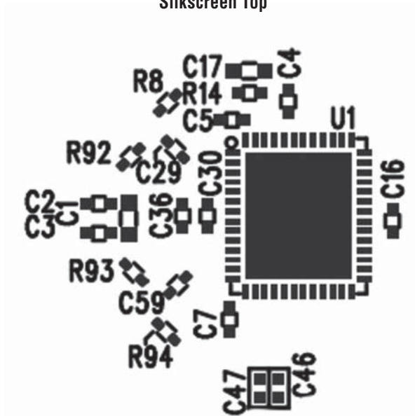
Silkscreen Top
