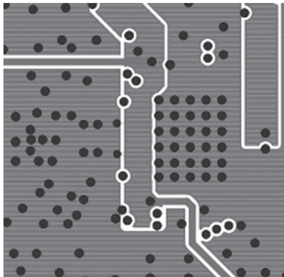
Inner Layer 5 Power
