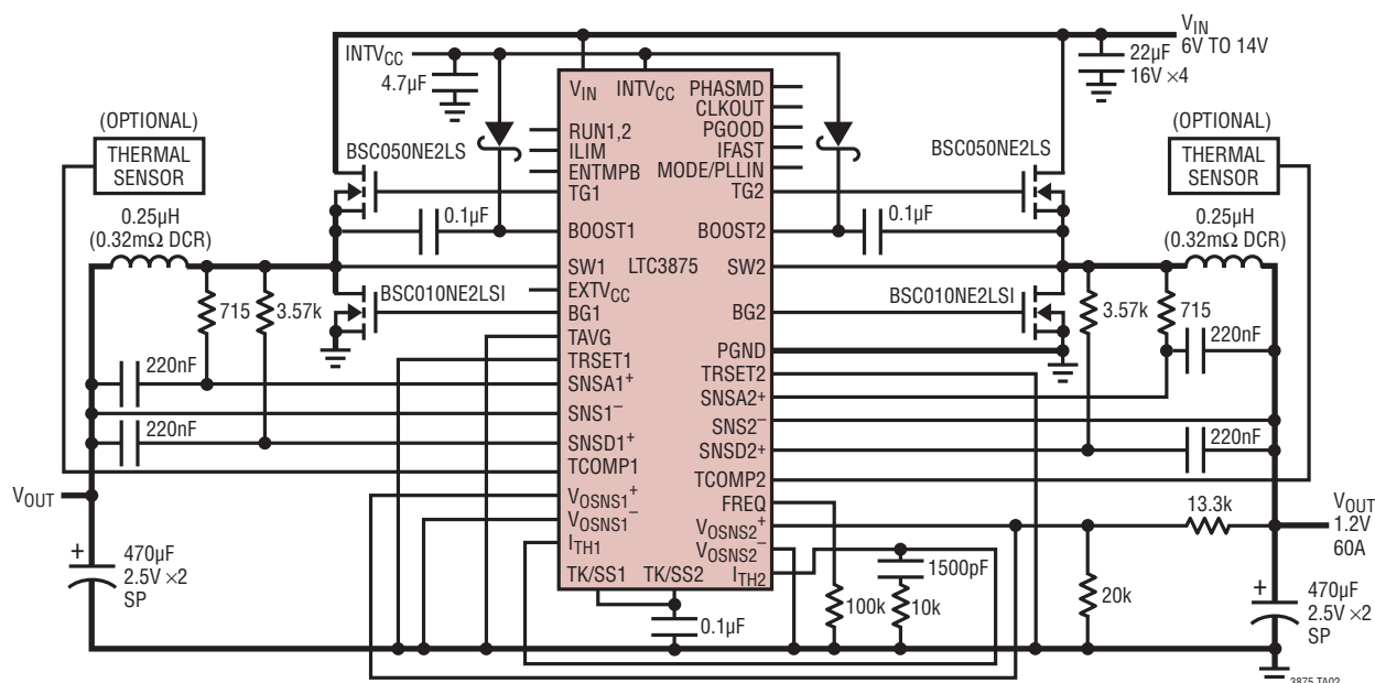
High Efficiency Dual Phase 1V/60A Step-Down Converter
