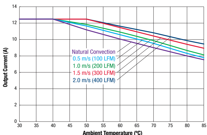
Maximum Current Temperature Derating at Sea Level (Vin = 75V, no baseplate. Airflow Direction Is Longitudinal from Vin to Vout.)
