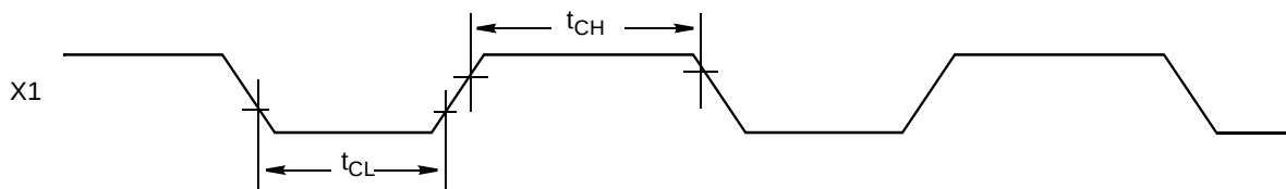
FIGURE 91. Clock Timing
