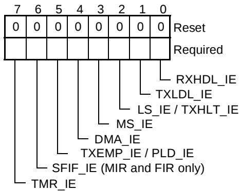
Event Identification Register (EIR) Bank 0, Offset 02h
