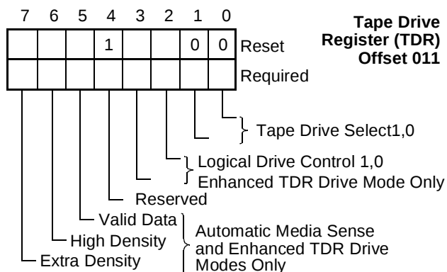
FIGURE 48. TDR Register Bitmap
