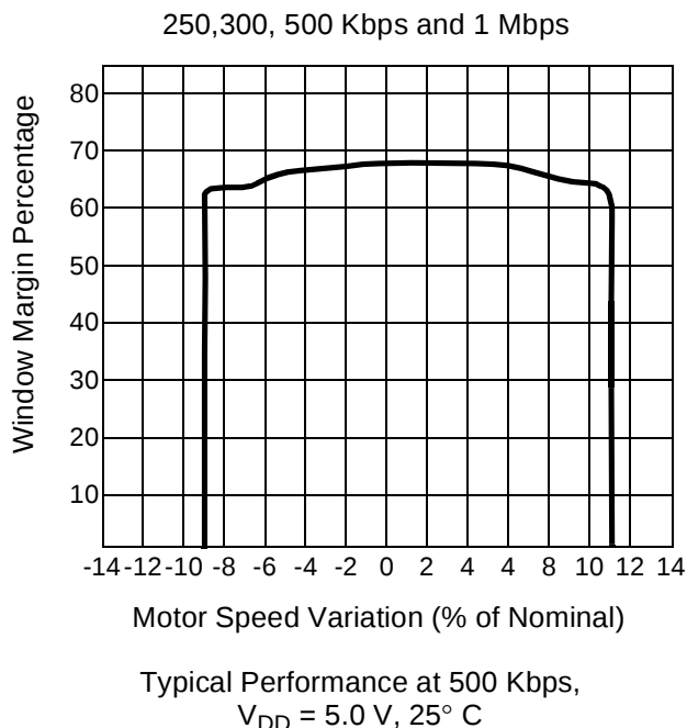
FIGURE 42. PC87338/PC97338 Dynamic Window Margin Performance
