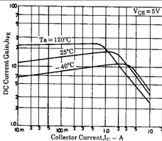
Fig.4 DC current Gain
