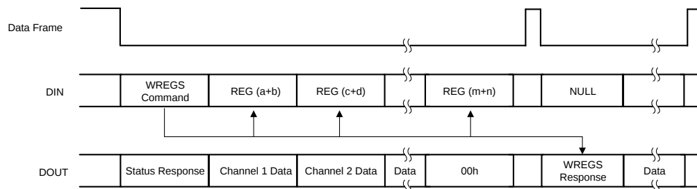
Figure 78. WREGS Command Status Response (Multiple Register Write)
