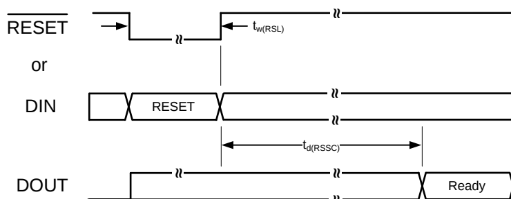
Figure 7. RESET Pin and Command Timing
