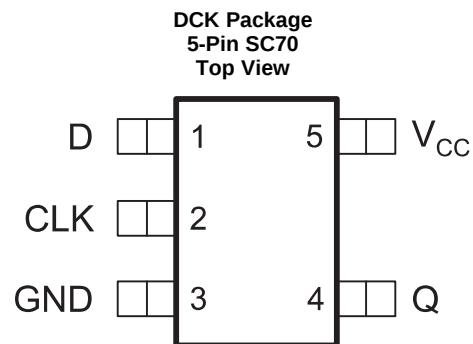
Pin Functions
