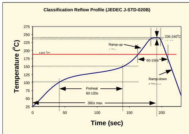
Fig 10. Recommended IR-reflow Soldering Profile
