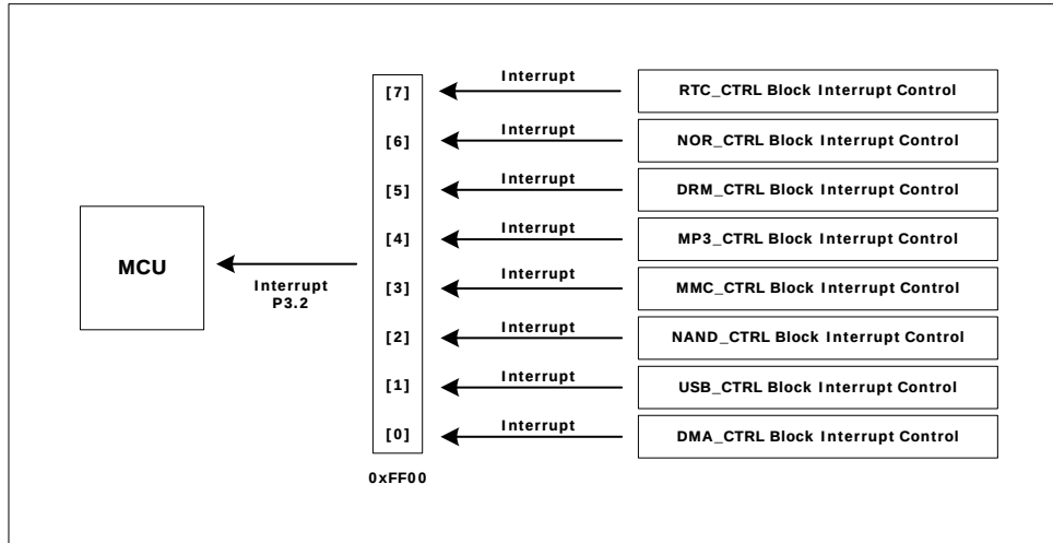
Figure 7. External Interrupt Mask to MCU
