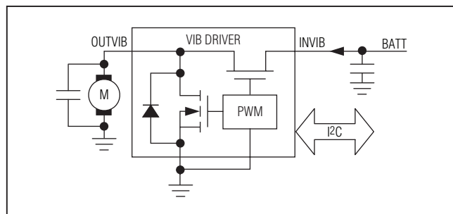
Figure 7. Vibrator Driver
