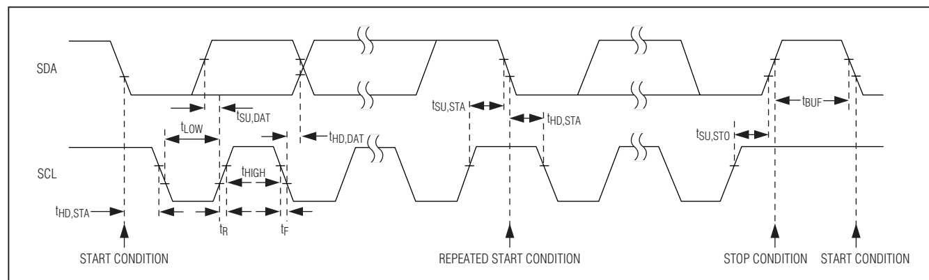
Figure 15. I 2 C Timing Diagram
