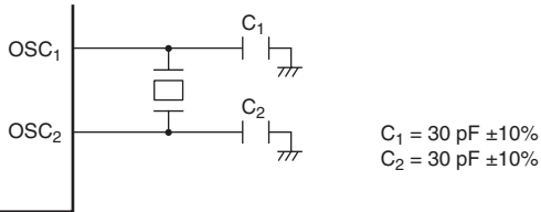
Figure 5.5 Typical Connection to Ceramic Resonator
