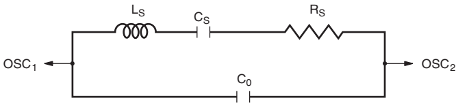
Figure 5.4 Equivalent Circuit of Crystal Resonator
