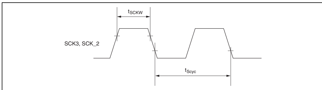
Figure 18.4 SCK3 Input Clock Timing
