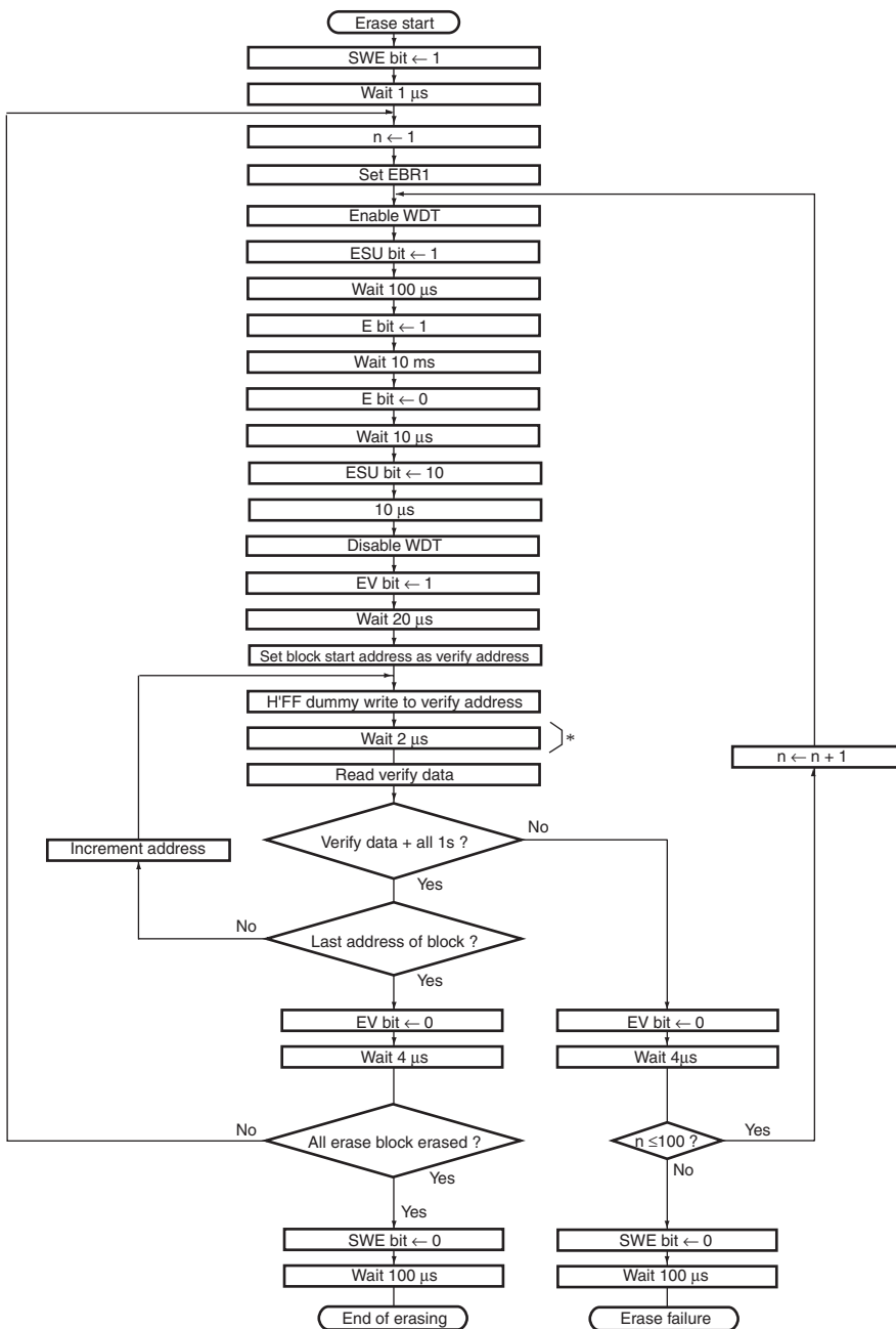
Figure 7.4 Erase/Erase-Verify Flowchart
