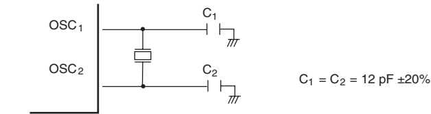
Figure 5.3 Typical Connection to Crystal Resonator
