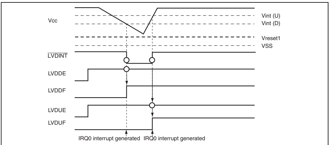
Figure 15.4 Operational Timing of LVDI Circuit
