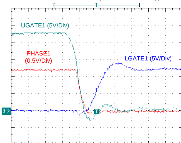
Gate Waveforms (UGATE Falling)
