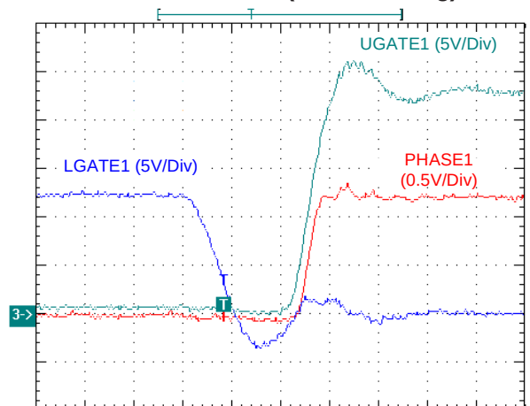
Gate Waveforms (UGATE Rising)
