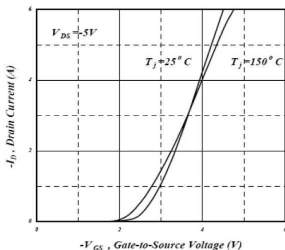
Fig 11. Transfer Characteristics
