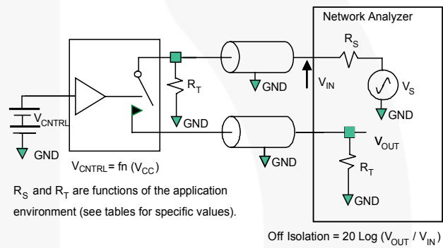
Figure 15. Channel Off Isolation
