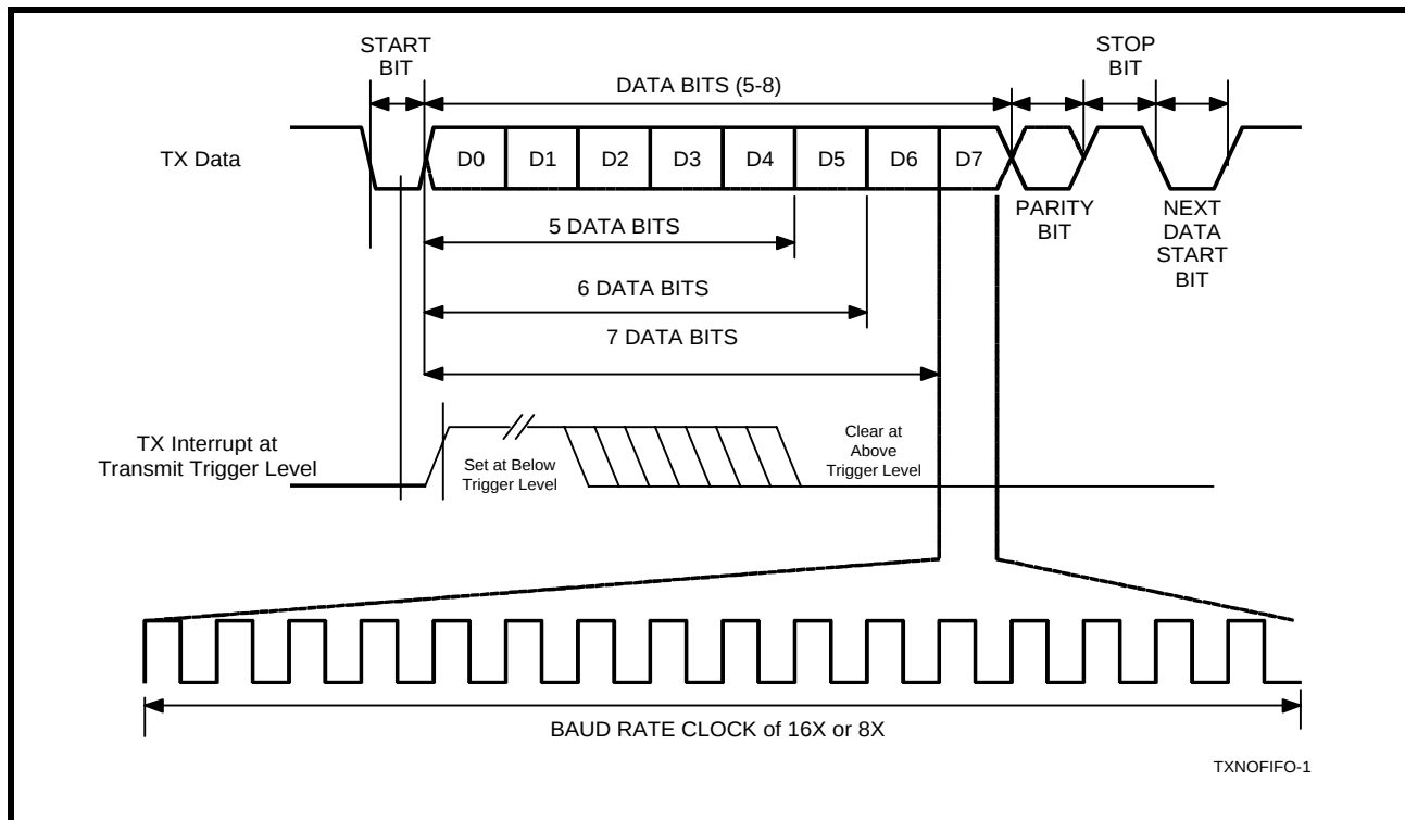
FIGURE 21. TRANSMIT DATA INTERRUPT AT TRIGGER LEVEL
