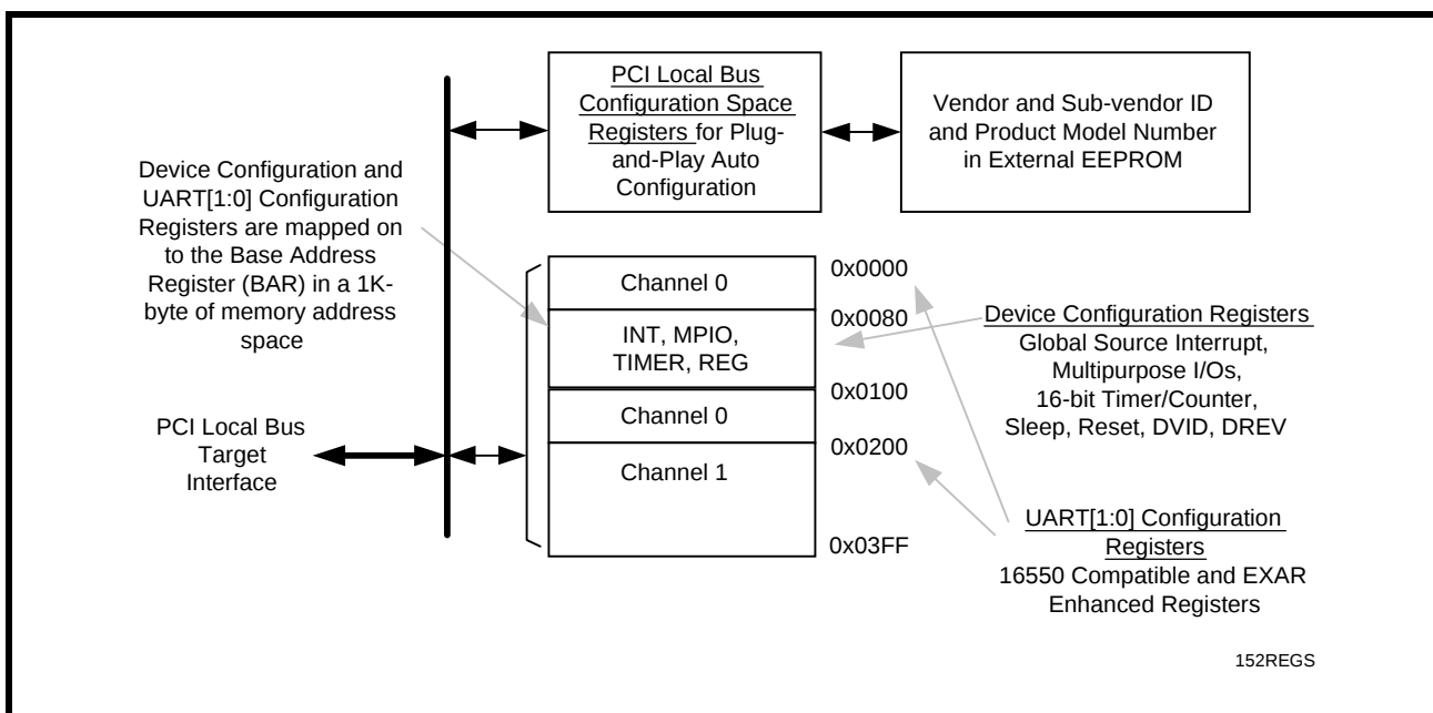
FIGURE 3. THE XR17L152 REGISTER SETS
