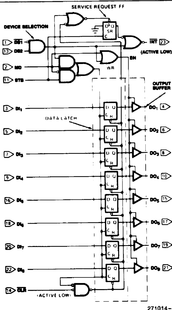
Figure 1. Logic Diagram
