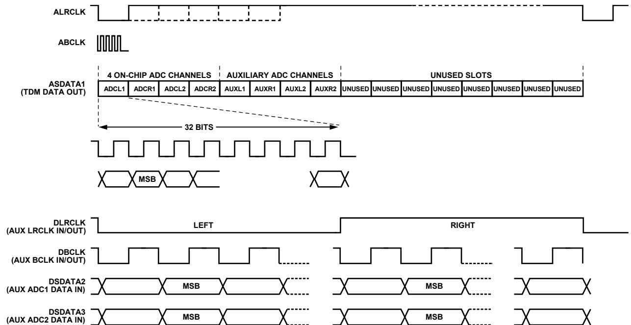
Figure 20. TDM/AUX Mode 16-Channel ADC Configuration
