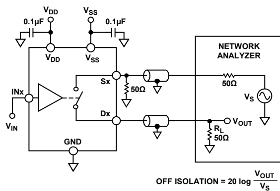
Figure 26. Off Isolation
