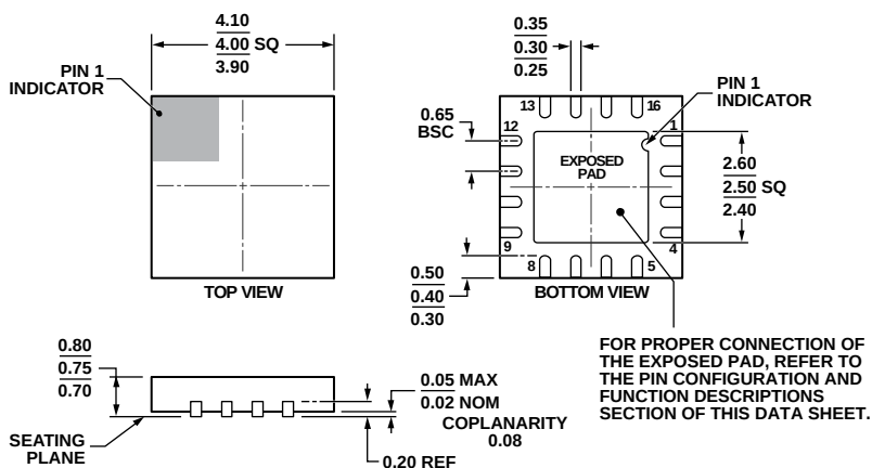
Figure 34. 16-Lead Lead Frame Chip Scale Package [LFCSP] 4 mm × 4 mm Body and 0.75 mm Package Height (CP-16-26) Dimensions shown in millimeters
