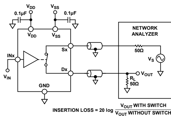
Figure 28. Bandwidth
